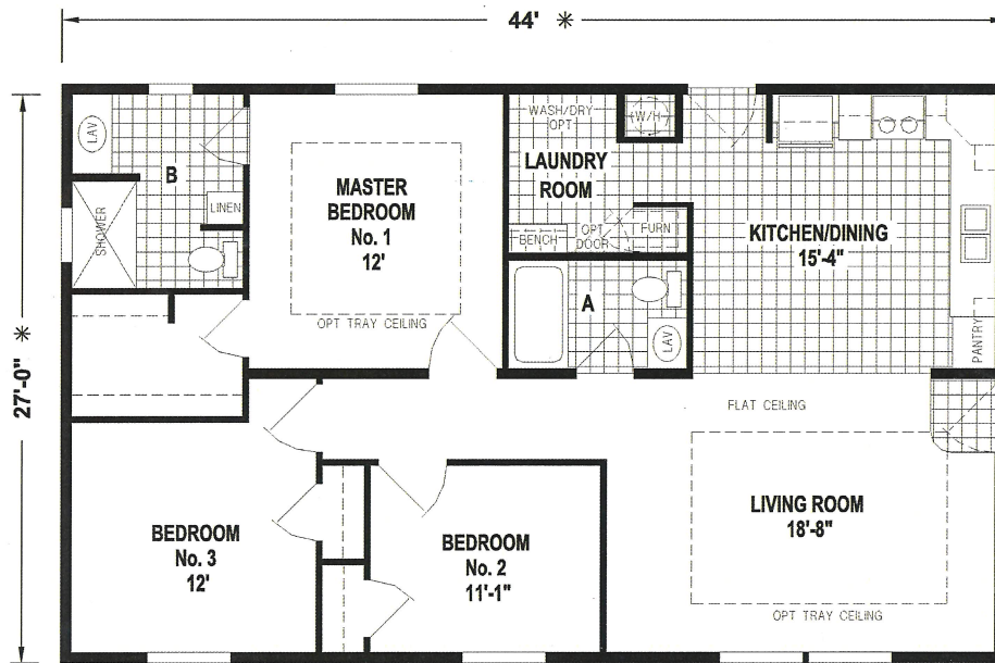
7550/4428 (1,144 SQ. FT.) 3BEDROOM - 2BATHS
